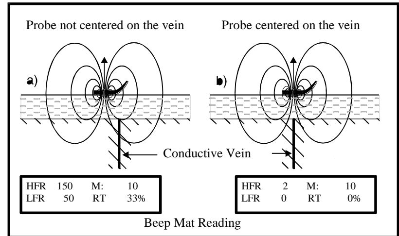
Illustration 18: Narrow conductor
